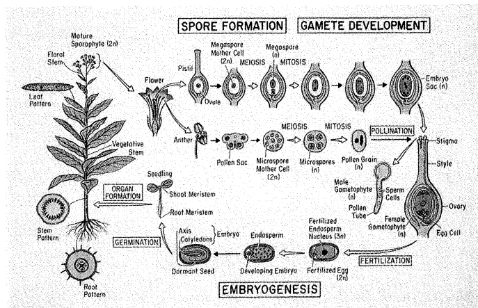
Fig. 1. Life cycle of a flowering plant.
