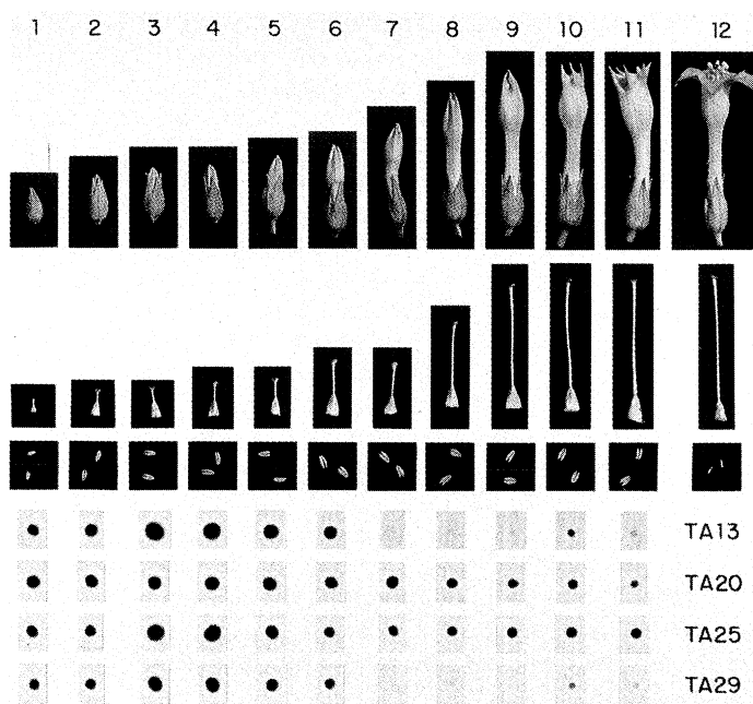
Fig. 5. Regulation of gene expression during tobacco flower development. Tobacco flower development was divided into 12 stages, with floral bud and petal lengths as developmental markers (40). In general, the transition from stage 1 to stage 12 occurred over a 1- to 2-week period depending on the time of year. Stage 1 and stage 12 flowers averaged 0.8 cm and 4.6 cm in length, respectively. Anther mRNAs were isolated from 12 stages of flower development, spotted onto Nytran membranes, and hybridized with labeled anther cDNA clones (40). TA13 and TA29 cDNA clones represent divergent mRNAs of the same gene family (40). By contrast, TA20 and TA25 cDNA clones represent unique anther mRNAs. At their peak levels, TA13, TA29, TA20, and TA25 mRNAs represent 0.42%, 0.26%, 0.48%, and 0.23% of the anther mRNA mass, respectively (40). TA13, TA25, and TA29 mRNAs are not detectable in heterologous vegetative and floral organ system mRNA populations. TA20 mRNA is represented at lower prevalences in pistil and petal mRNAs.
