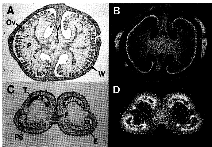
Fig. 6. Localization of mRNAs in the tobacco anther and ovary. Stage 6 ovaries and stage 4 anthers (Fig. 5) were fixed, embedded in paraffin, and hybridized in situ with single-stranded ^{35}\text{S} -labeled RNA probes (15–17). (A and B) Hybridization of an ovary cross section with the TA20 probe (Fig. 5). The TA20 mRNA is approximately 20% less prevalent in the pistil than in the anther (40, 41). (A) Bright-field photograph. (B) Dark-field photograph. White grains represent regions containing RNA/RNA hybrids. (C and D) Hybridization of an anther cross section with the TA29 probe (Fig. 5). (C) Bright-field photograph. (D) Dark-field photograph. White grains represent regions with RNA/RNA hybrids. Abbreviations: Ov, ovule; P, placenta; V, vascular tissue; W, ovary wall; PS, pollen sac; T, tapetum; and E, endothecium.
