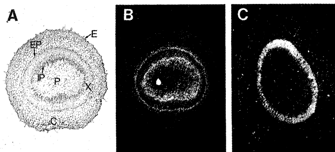
Fig. 2. Localization of mRNAs in the tobacco stem. Floral stems were fixed, embedded in paraffin, and hybridized in situ with single-stranded 32 S-labeled RNA probes (15–17). (A) Bright-field photograph. E, epidermis; C, cortex; P, pith; X, xylem; EP, external phloem; and IP, inner phloem. (B) Hybridization with the TS13 probe (18). TS13 represents a 0.7-kb mRNA that is present at high levels in the stem but is detectable at lower levels in heterologous organ systems (19). Photograph was taken by dark-field microscopy. The white grains represent regions containing RNA/RNA hybrids. (C) Hybridization with the TP7 probe (18). TP7 represents a 1.4-kb mRNA that is present at high levels in the stem and petal but is also detectable at lower concentrations in other organ systems (20). Dark-field micrograph as in (B). RNA/RNA hybrids are indicated by the white grains.
