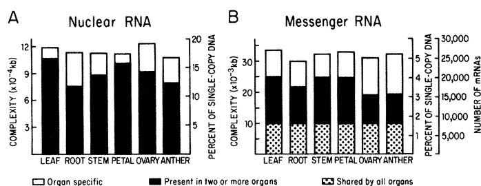
Fig. 3. Regulation of gene expression in flowering plants. Data represent the results of solution RNA-excess hybridization experiments with tobacco single-copy DNA and were taken from Kamalay and Goldberg (21, 22). Complexity values were calculated by using a tobacco single-copy DNA complexity of 6.4 \times 10^5 kb (21). (A) Hybridization with nuclear RNA populations. Total nuclear RNA [poly(A) + and poly(A) - ] was used for these experiments (22). In general, the nuclear RNA/mRNA complexity ratio for any given organ system is approximately 3.6. (B) Hybridization with mRNA populations. Experiments were performed with total polysomal RNA [poly(A) + and poly(A) - ] that was released from polysomes with EDTA (21). The number of diverse mRNA species in each mRNA population was calculated by assuming an average transcript size of 1.2 kb (21). Leaf and petal mRNA sets are qualitatively indistinguishable from each other in population hybridization experiments (21). Leaf and petal white bar areas represent mRNA species that are present in both the leaf and petal but are undetectable in heterologous organ system mRNAs. Recent experiments with petal cDNA clones indicate that there are quantitative differences with respect to specific mRNA species in the leaf and petal (20).
