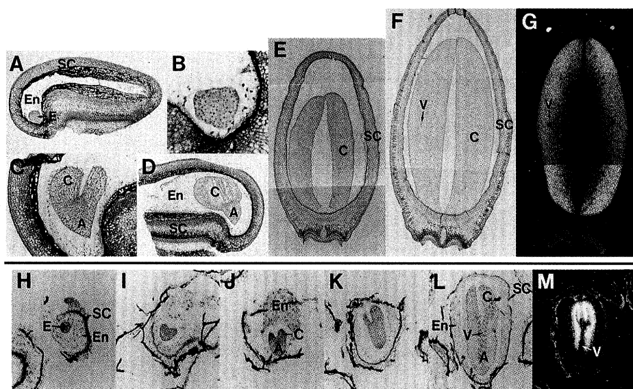
Fig. 4. Localization of seed protein mRNA in soybean and transformed tobacco seeds. (A–F) Bright-field photographs of soybean seed development (31). (A and B) Globular embryo, (C) heart stage embryo, (D) cotyledon stage embryo, (E and F) maturation-stage embryos. (G) In situ hybridization of a labeled single-stranded lectin RNA probe with a longitudinal section of a maturation stage soybean embryo (16, 17). The photograph was taken by dark-field microscopy, and the white grains represent regions with RNA/RNA hybrids. (H to L) Bright-field photographs of tobacco seed development. Tobacco seed development was characterized by Barker and Goldberg (16). (H) Globular stage embryo, (I and J) heart-stage embryos, (K and L) torpedo or maturation-stage embryos. (M) In situ hybridization of a labeled lectin mRNA probe with a longitudinal section of a transformed tobacco seed containing a soybean lectin gene (37). The photograph was taken by dark-field microscopy (16, 17). Abbreviations: E, embryo; En, endosperm; SC, seed coat; C, cotyledon; A, axis; and V, vascular tissue.
