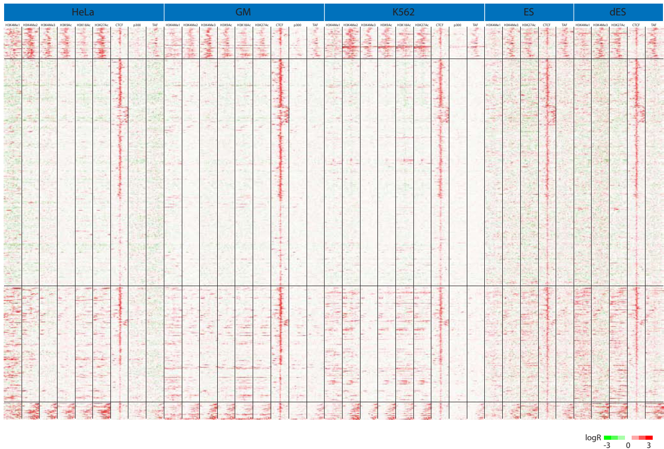
Figure S11: Chromatin features at CTCF binding sites.
