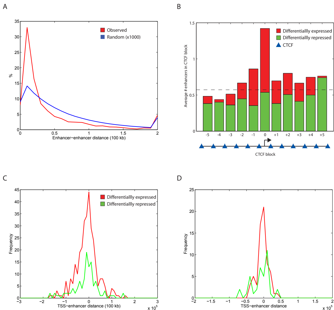
Figure S13: ENCODE Enhancers are clustered at differentially expressed genes.
