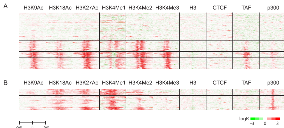
Figure S9: Chromatin acetylation features at promoters and enhancers in the ENCODE regions.
