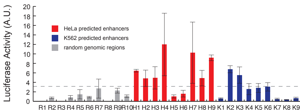
Figure S7: Cell type-specificity of predicted enhancer activity in reporter assays
