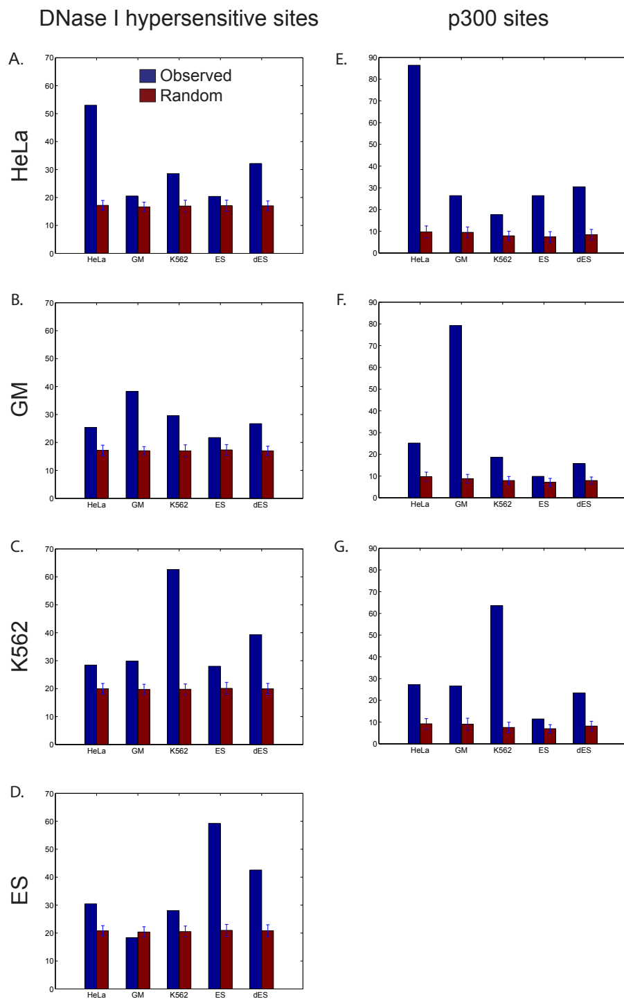
Figure S3: Verification of histone modification-based prediction of enhancers in the ENCODE regions
