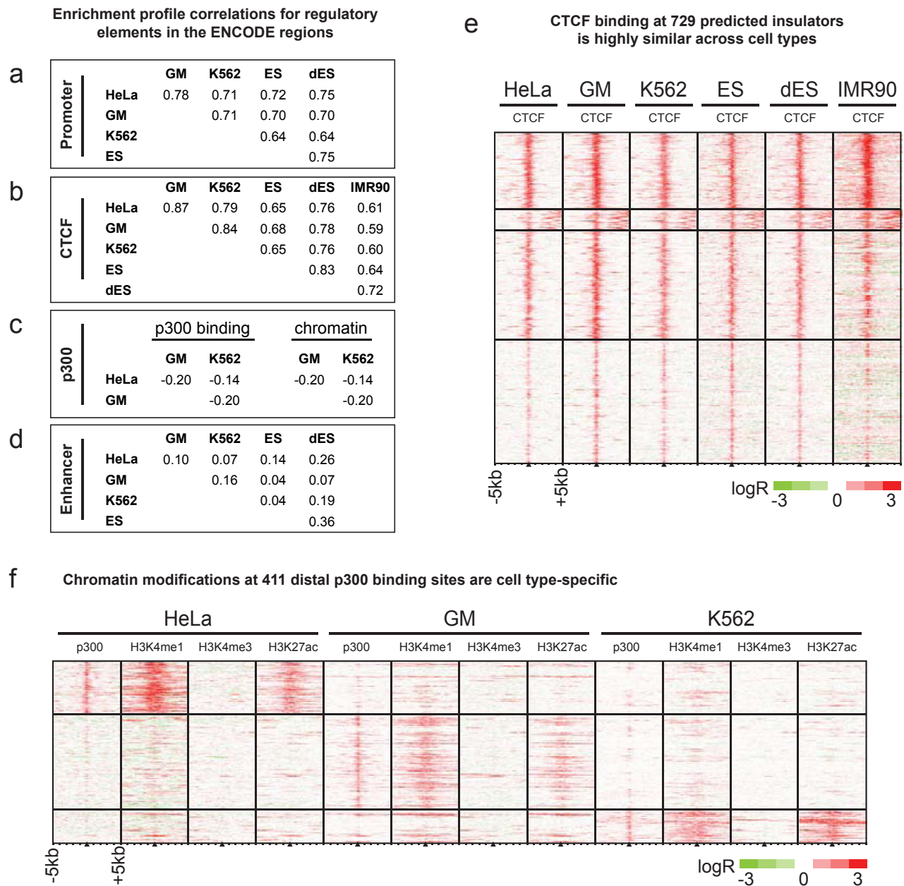
Figure S1: Quantitative comparison of regulatory elements in the ENCODE regions
