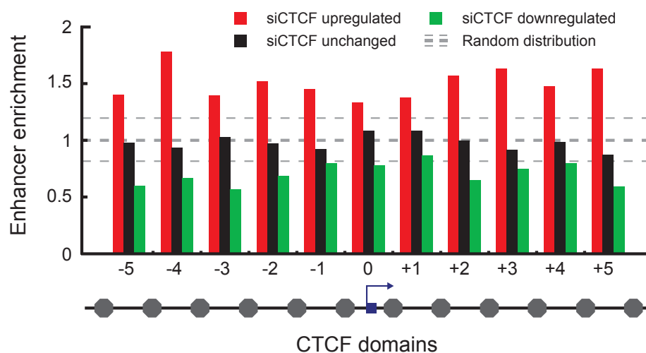
Figure S14: CTCF sites may serve as domain boundaries for promoter-enhancer interactions
