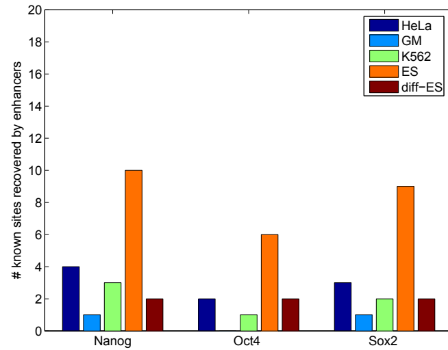
Figure S4: Predicted ES enhancers are enriched in known ES-specific transcription factors
