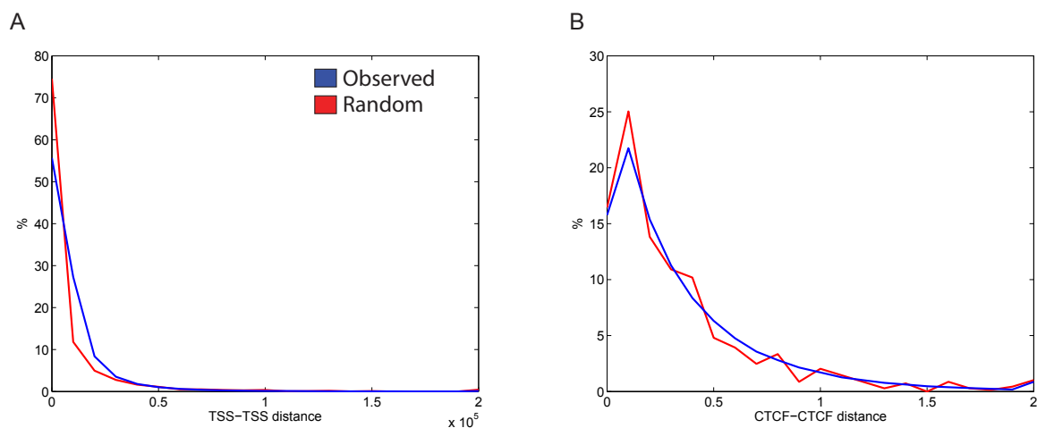
Figure S12: Distribution of promoters and insulators in the ENCODE regions.
