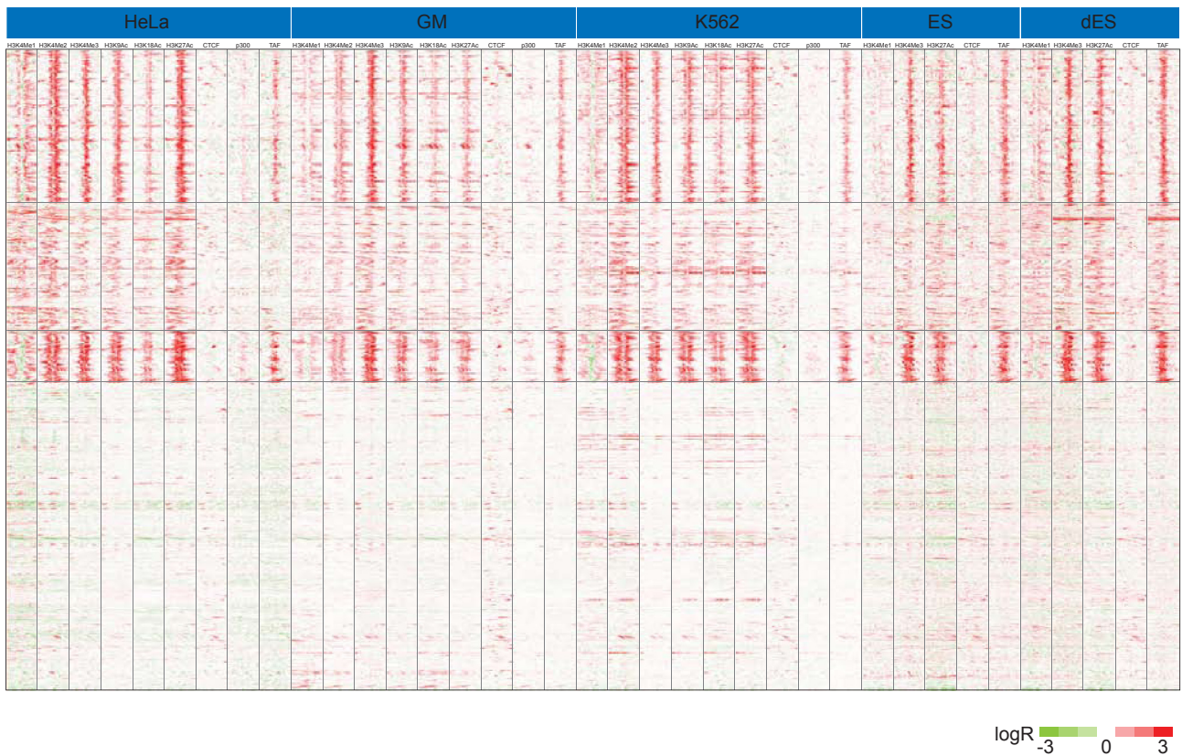
Figure S2: ChIP-chip enrichment profiles at Gencode promoters in the ENCODE regions
