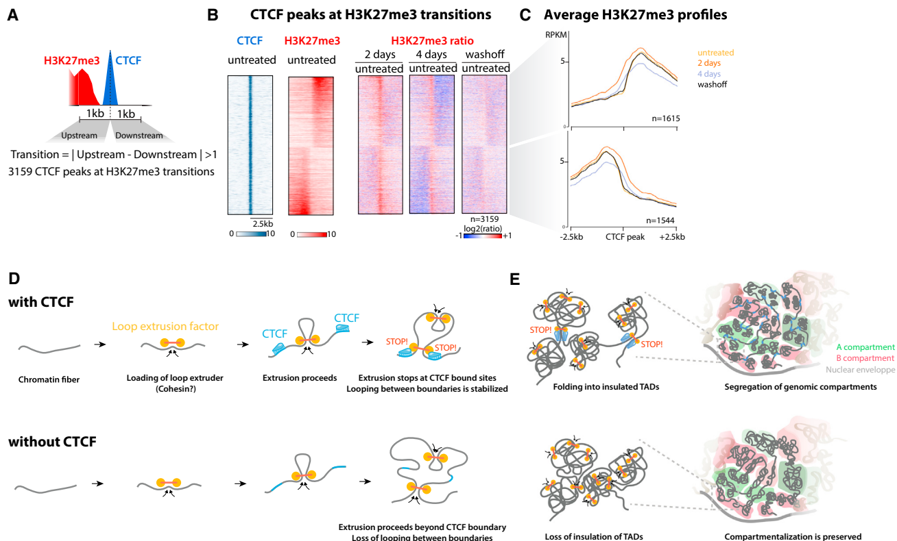
Figure 7. CTCF Does Not Constrain H3K27me3 Spreading in mESCs and Summary Model
