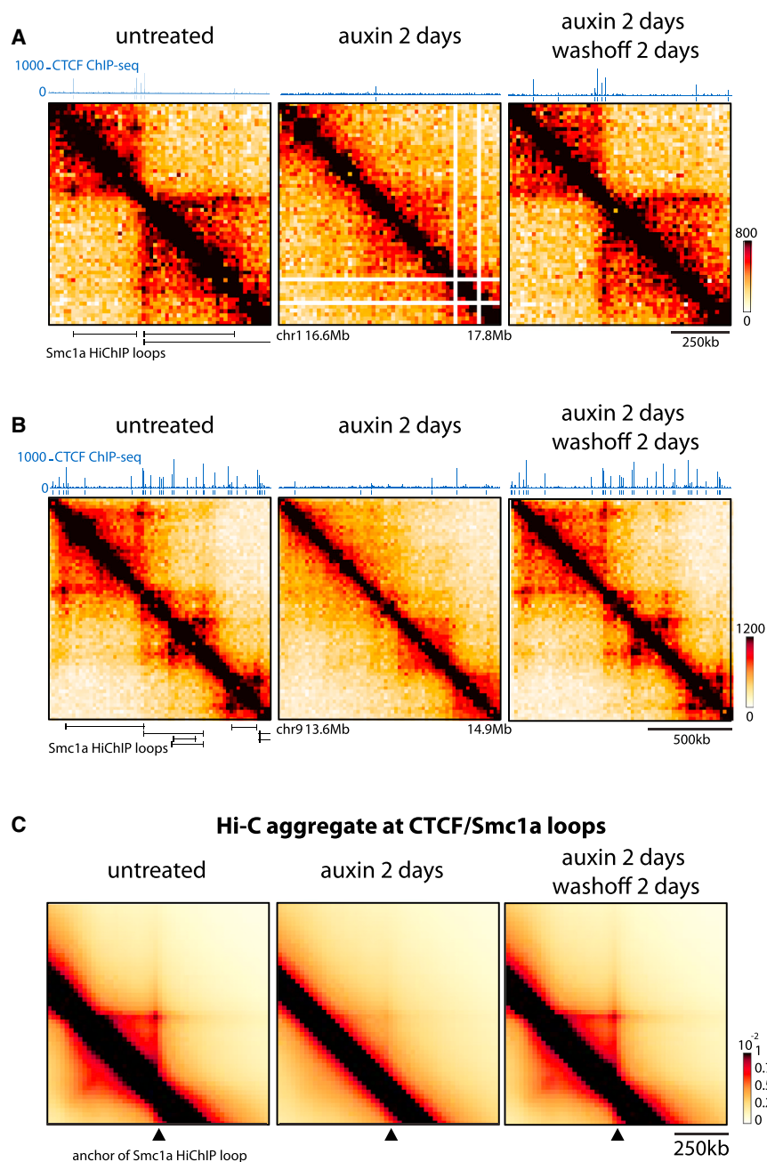
Figure 2. CTCF Is Required for Accumulating Loops between CTCF and Cohesin Binding Sites
