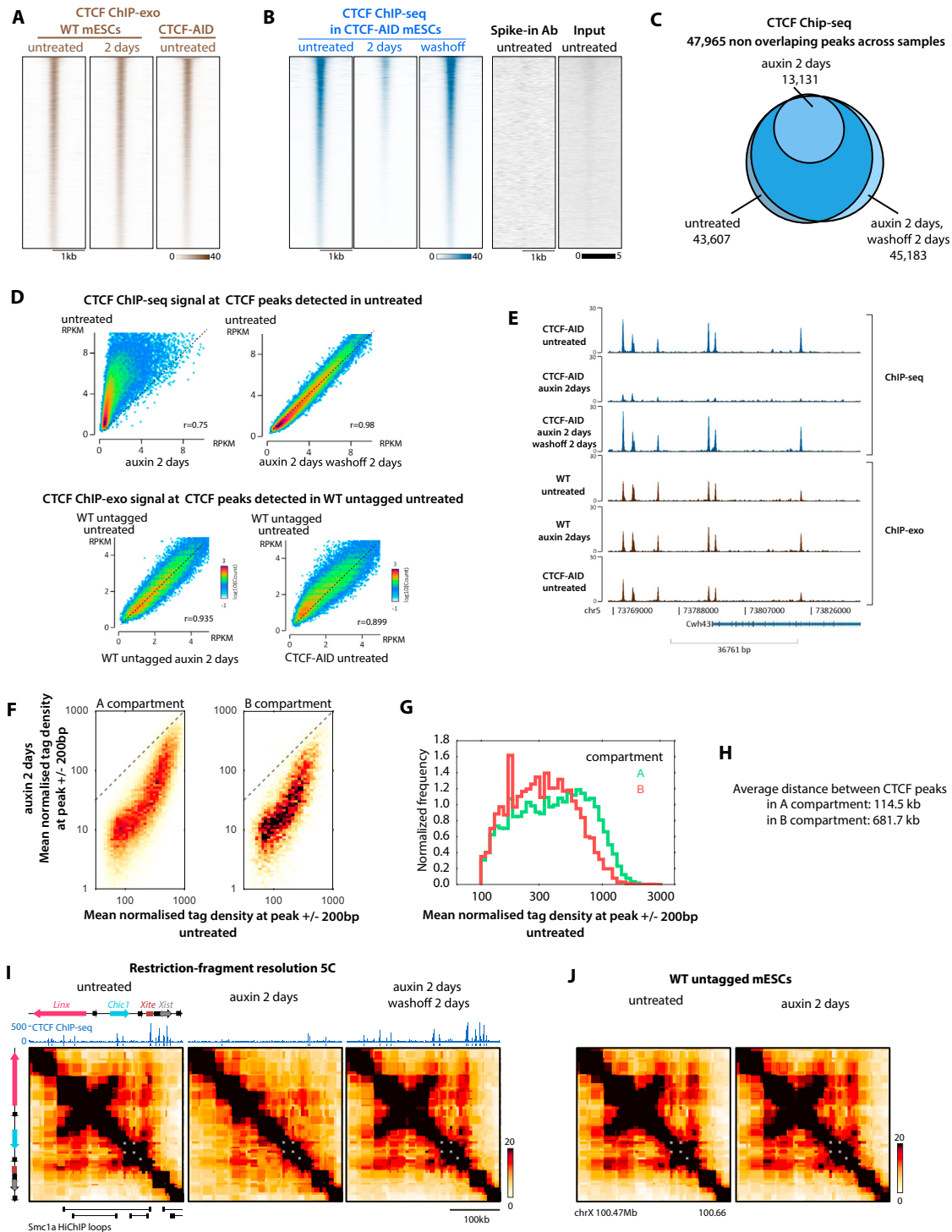
Figure S2. CTCF-ChIP-Seq Analysis and Chromosome Conformation Capture Carbon-Copy (5C), Related to Figure 2
