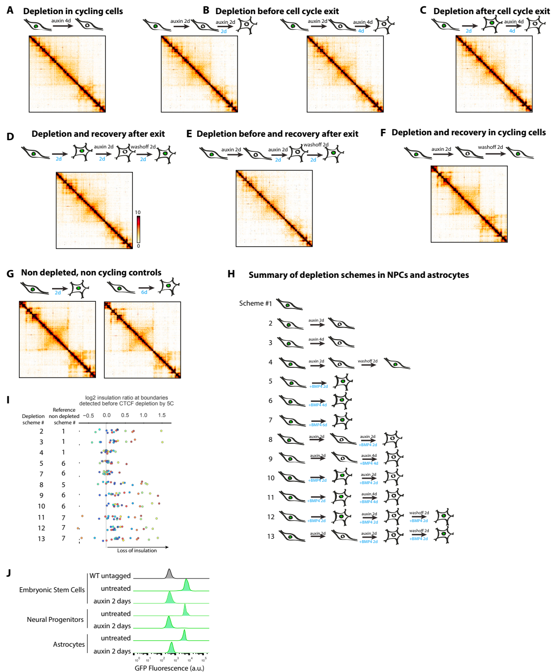
Figure S5. CTCF is Required for Proper TAD Folding in Differentiated and Non-cycling Cells, Related to Figure 5
