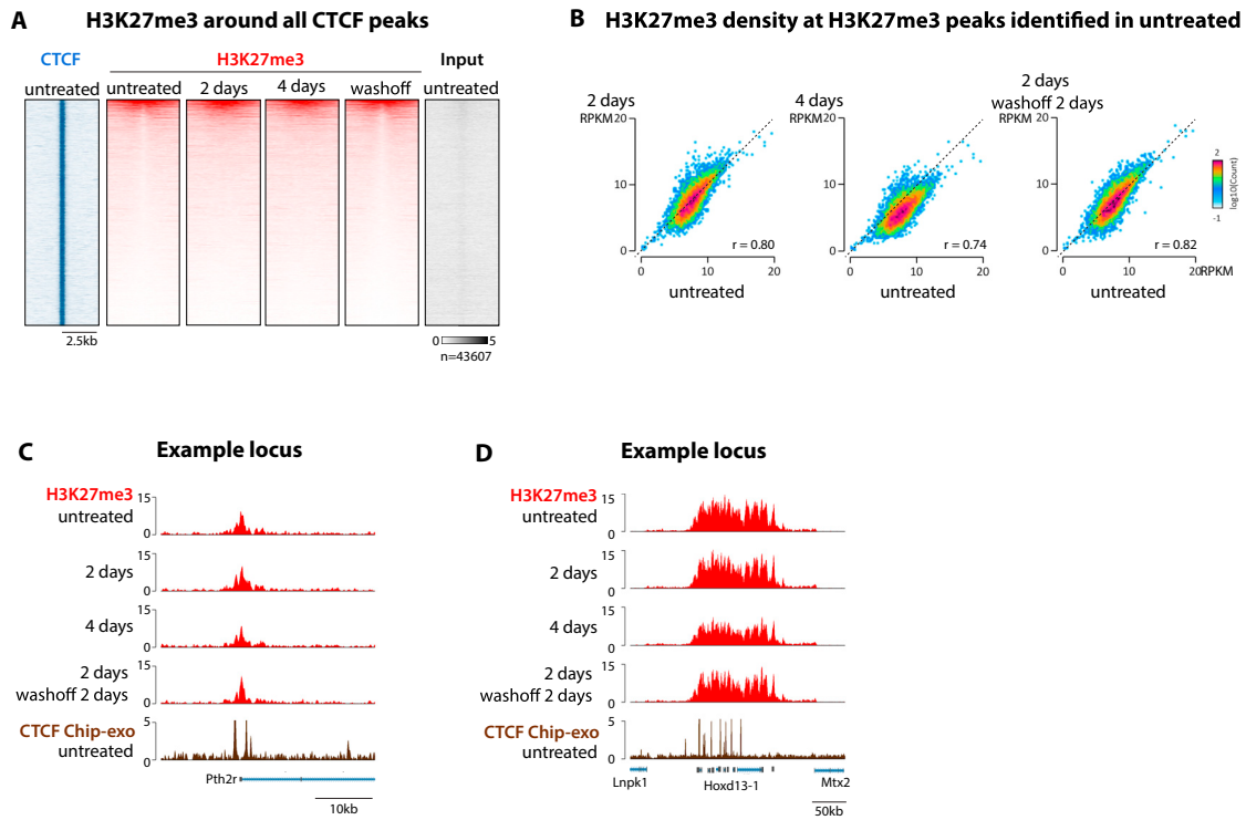
Figure S7. Additional Analyses of H3K27me3 Patterns after CTCF Depletion, Related to Figure 7
