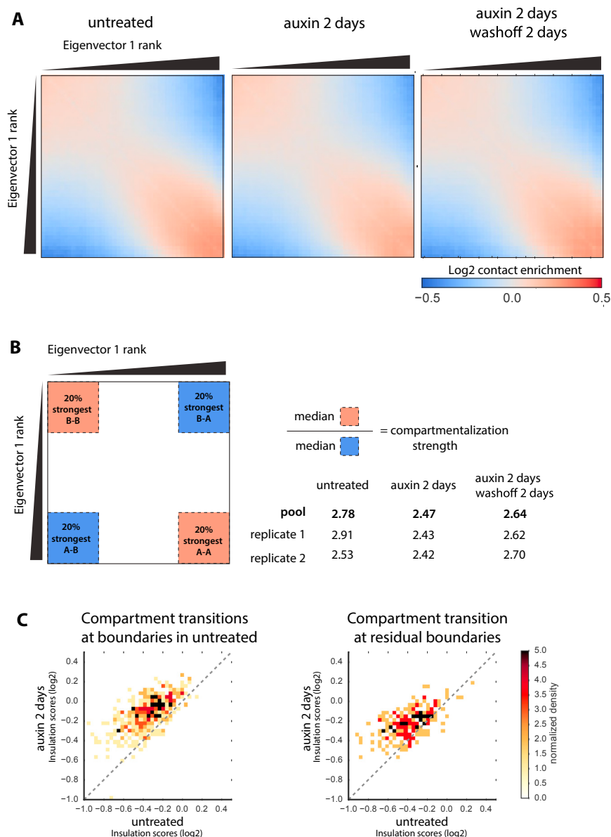
Figure S4. Large-Scale Chromosome Folding is Largely Unaffected by CTCF Depletion, Related to Figure 4
