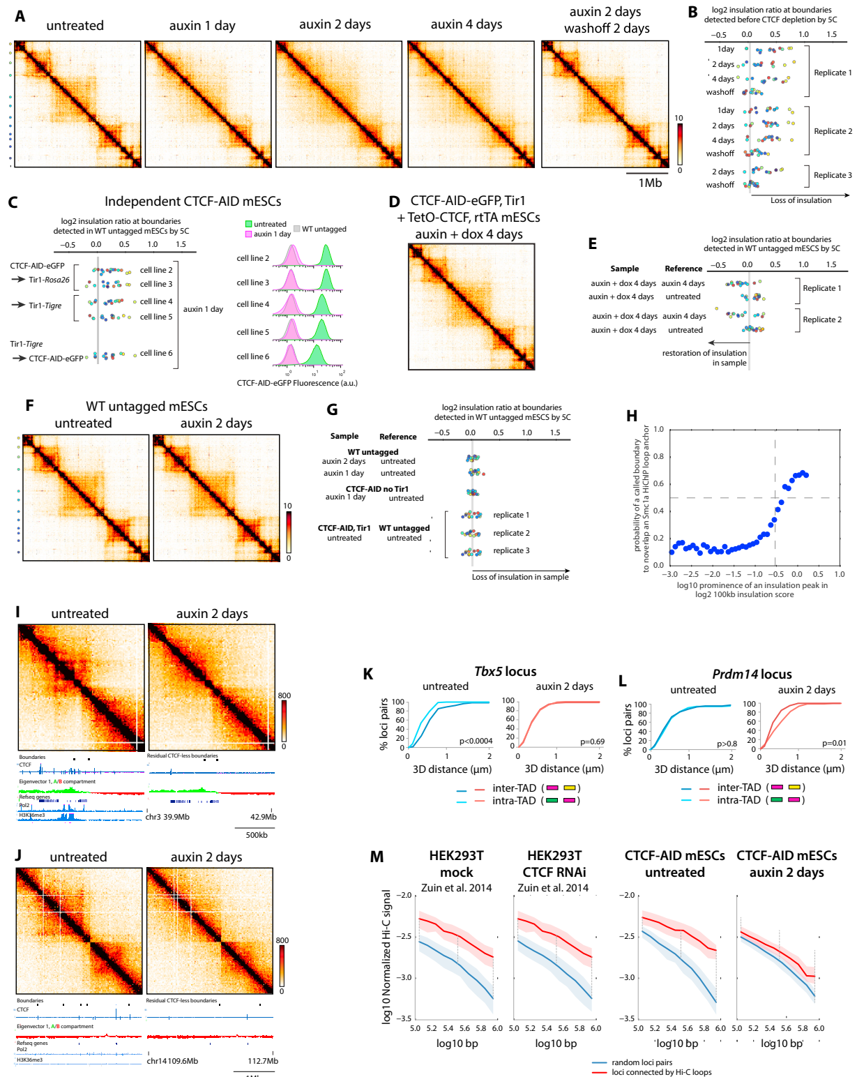
Figure S3. Supporting Data Regarding Loss of TAD Insulation upon CTCF Depletion, Related to Figure 3
