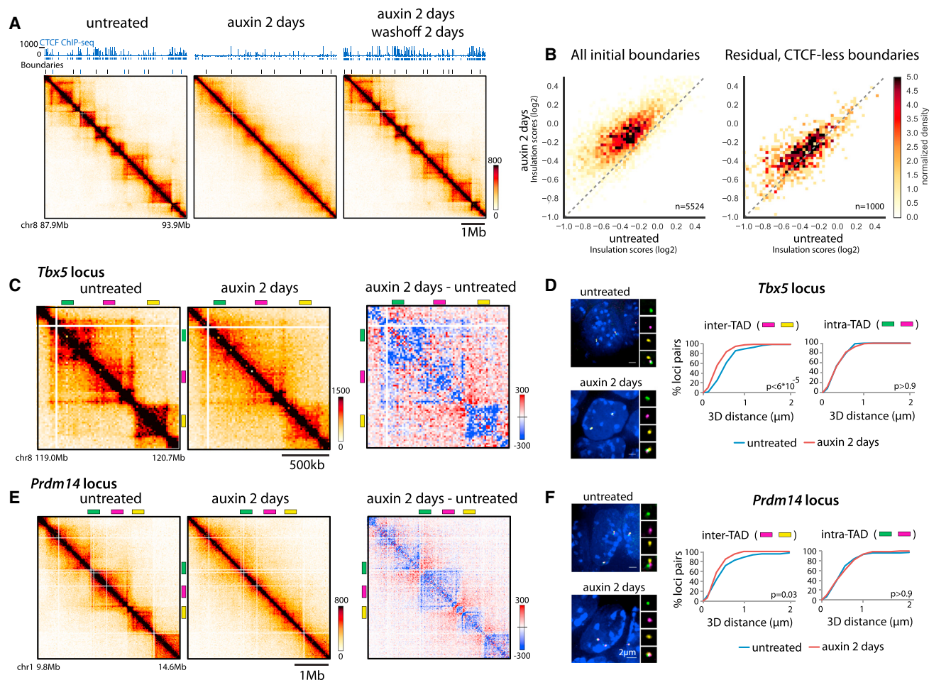
Figure 3. CTCF Instructs Insulation of TADs
