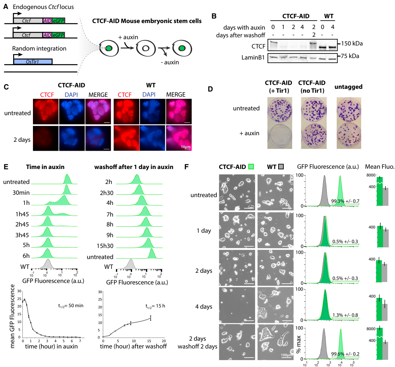
Figure 1. Acute and Reversible Depletion of CTCF with the AID System in mESCs
