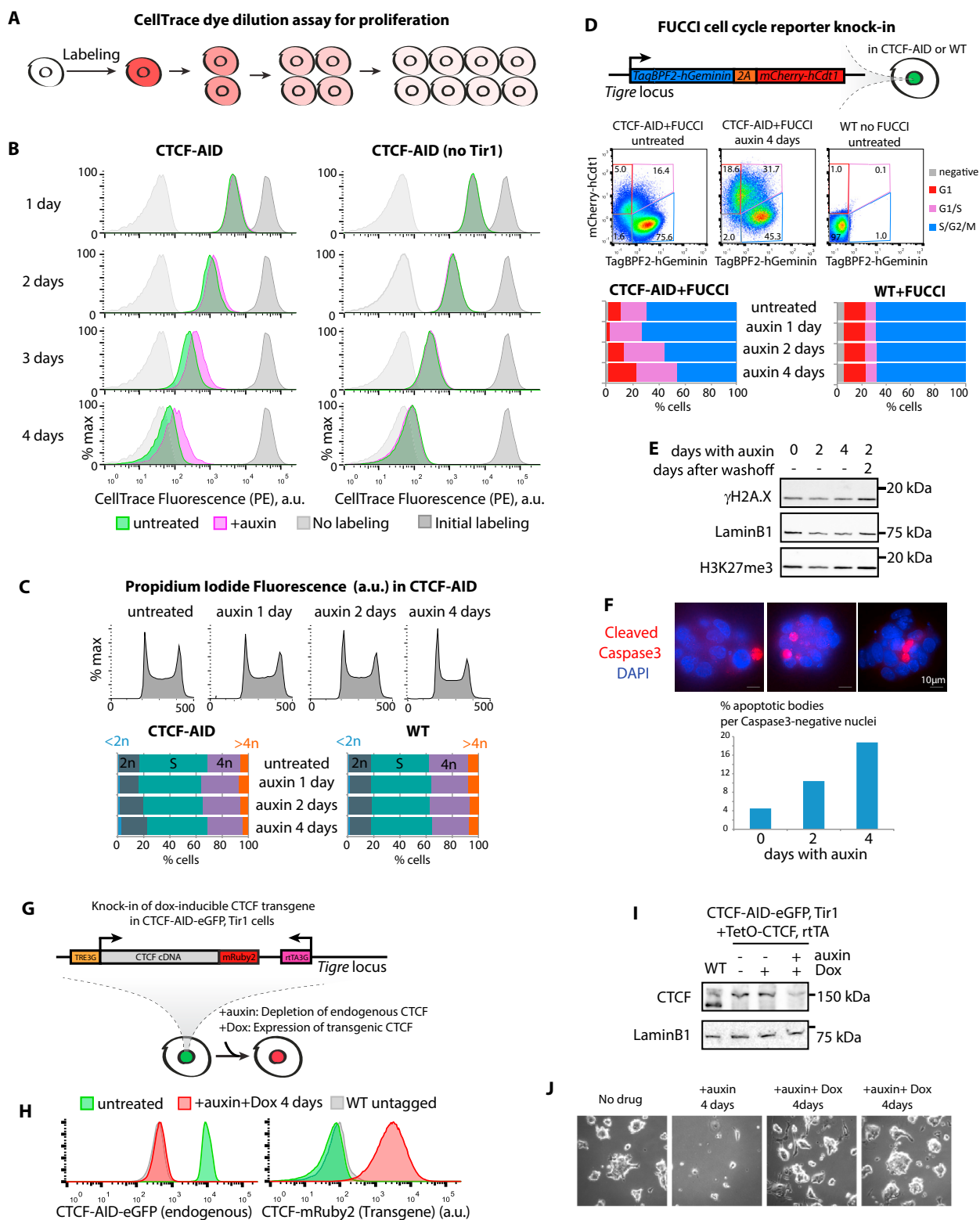
Figure S1. Characterization of the CTCF-AID mESCs, Related to Figure 1
