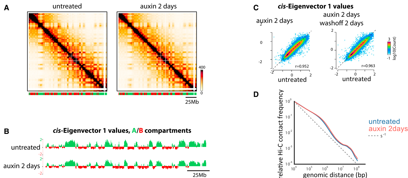
Figure 4. Proper Insulation of TADs Is Not Required for Higher-Order Segregation of A and B Compartments
