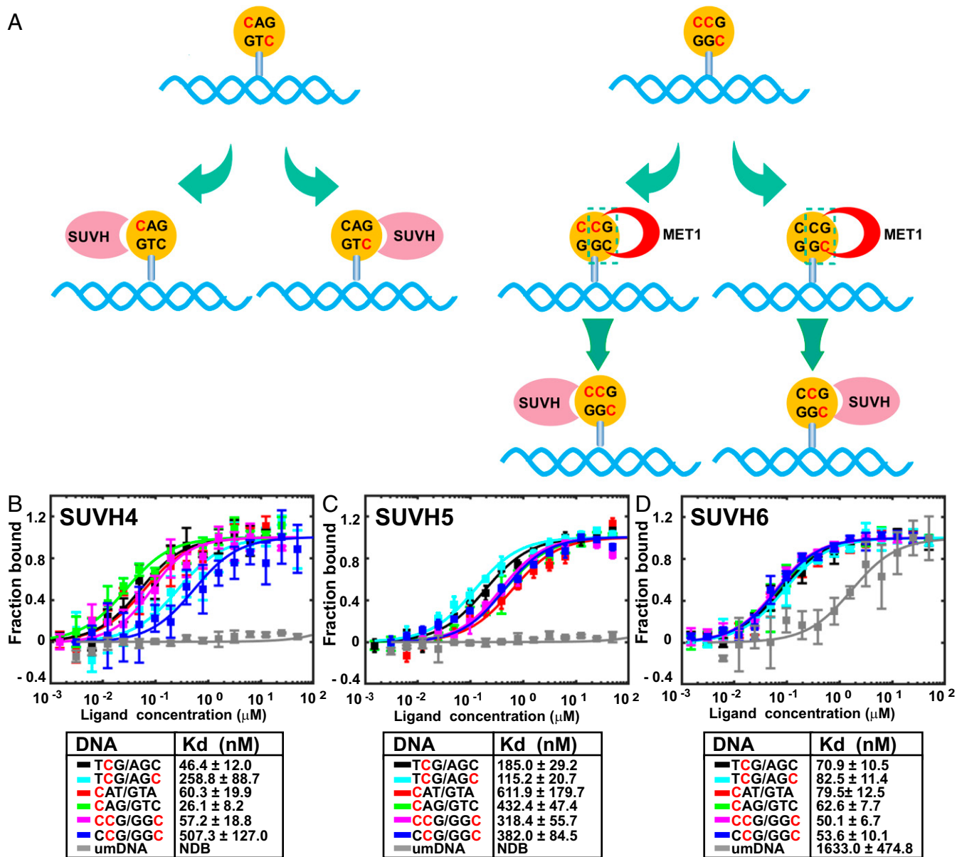
Fig. 4. The three SUVH proteins possess different mDNA binding preferences. (A) Schematic model of CHG methylated DNA during replication. CAG/GTC DNA generates CAG/GTC and CAG/GTC replication products which can be directly recognized by SUVH proteins (Left). CCG/GGC DNA could yield CCG/GGC and CCG/GGC replication products, which are methylated by MET1 to generate CG methylation and then serve as binding targets for the SUVH protein (Right). (B–D) Binding curves between different methylated DNAs and KYP (B), SUVH5 (C), and SUVH6 (D) measured by MST. Data points are shown as means ± SD ( n = 3 ). Curves indicate the calculated fits according to the data points, and the binding affinities ( K_d ) are listed in the boxes below the binding curves. DNA sequences can be found in SI Appendix, Table S2 . C marked in red in the sequence indicates 5mC. NDB, no detectable binding.
