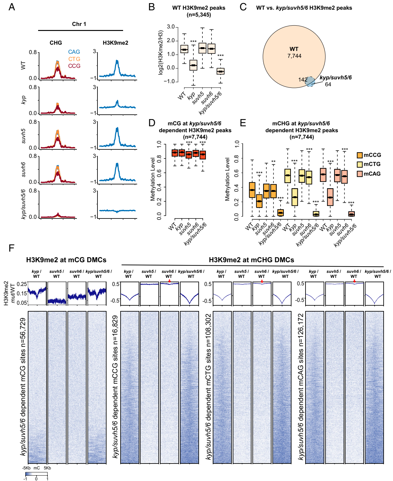
Fig. 5. Interdependent H3K9me2 and DNA methylation defects in kyp , suvh5 , suvh6 , and kyp/suvh5/6 . (A) Chromosomal distribution of CHG (mCAG, mCCG, and mCTG) methylation and log 2 ratio of H3K9me2/H3 in WT, kyp , suvh5 , suvh6 , and kyp/suvh5/6 in chromosome 1 (bin = 100 kb). (B) Boxplot of log 2 ratio of H3K9me2/H3 levels, at WT defined H3K9me2/H3 peaks (using callpeak function in MACS2), in WT, kyp , suvh5 , suvh6 , and kyp/suvh5/6 . *** P value <2.2e -16 , ** P value <1e -8 with Student's t test. (C) H3K9me2/H3 peak overlap defined by comparison between WT and kyp/suvh5/6 (using bdgdiff in MACS2). (D) Boxplot for CG methylation levels in WT, kyp , suvh5 , suvh6 , and kyp/suvh5/6 at kyp/suvh5/6 -dependent H3K9me2/H3 peaks [defined by H3K9me2 peaks called in WT but not in kyp/suvh5/6 (n = 7,744), see C]. *** P value <2.2e -16 , ** P value <1e -8 with Student's t test. (E) Boxplot for CHG methylation (mCCG, mCTG, and mCAG) levels of kyp/suvh5/6 -dependent H3K9me2/H3 peaks in WT, kyp , suvh5 , suvh6 , and kyp/suvh5/6 . *** P value <2.2e -16 , ** P value <1e -8 with Student's t test. (F) Heatmap of normalized H3K9me2 levels in kyp /WT, suvh5 /WT, suvh6 /WT, and kyp/suvh5/6 /WT plotted over kyp/suvh5/6 -dependent CG and CHG sites (mCCG, mCTG, and mCAG). Red arrows indicate H3K9me2 depletion in suvh6 centered on DMCs.
