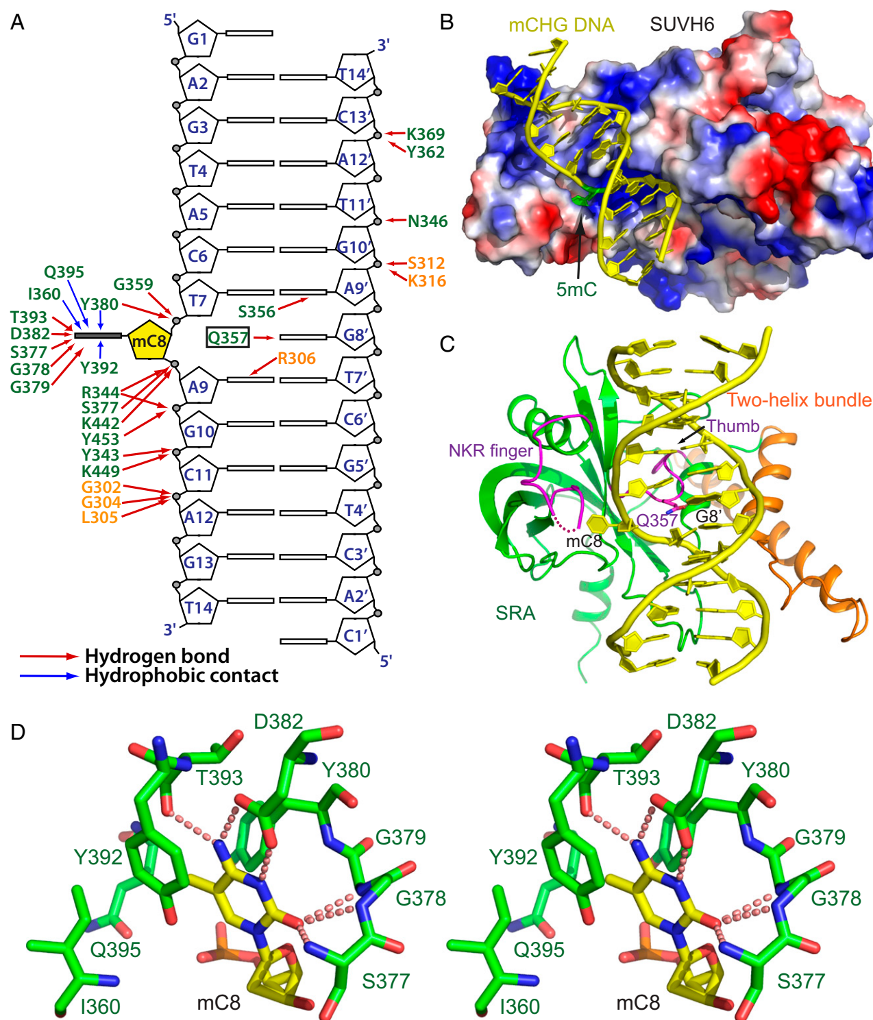
Fig. 3. Molecular basis for the recognition of mCHG DNA by SUVH6. (A) Schematic showing details of the interaction between SUVH6 and mCHG DNA. The residues of the two-helix bundle and the SRA domain are colored in orange and green, respectively. Hydrogen bonds and hydrophobic contacts are shown in red and blue arrows, respectively. (B) Electrostatic surface representation of SUVH6 with the mCHG DNA in ribbon representation showing that the DNA binds in a positively charged surface groove. The mC8 residue is highlighted in green and inserts into a small pocket of the SRA domain. (C) Structural mechanism for the flipping out of 5mC8 by SUVH6. The two-helix bundle, the SRA, and DNA are colored in orange, green, and yellow, respectively. The thumb loop and NKR finger loop are highlighted in magenta. Gln357 of the thumb loop occupies the gap left by the flipped-out 5mC8 and forms hydrogen bonds with the orphaned G8'. The NKR finger loop is partially disordered as shown by a dashed line. (D) Stereoview of the details of the specific recognition of the flipped-out 5mC base. Hydrogen bonds are highlighted by dashed red lines.
