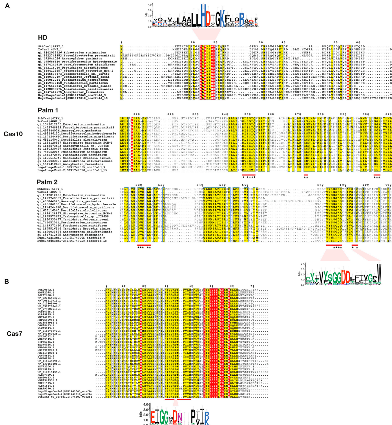
Figure S1. Sequence similarity of phage-encoded CRISPR-Cas systems, related to Figure 3
