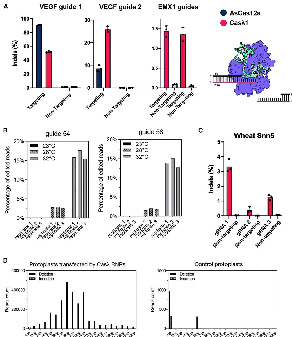
Figure 5. Casλ RNPs are functional for editing endogenous genes in human, Arabidopsis , and wheat cells with large deletion profiles
