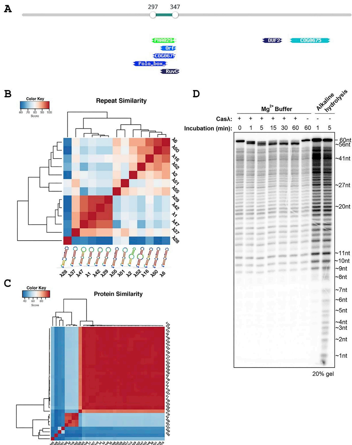
Figure S3. Divergent properties of Casλ, related to Figure 4
