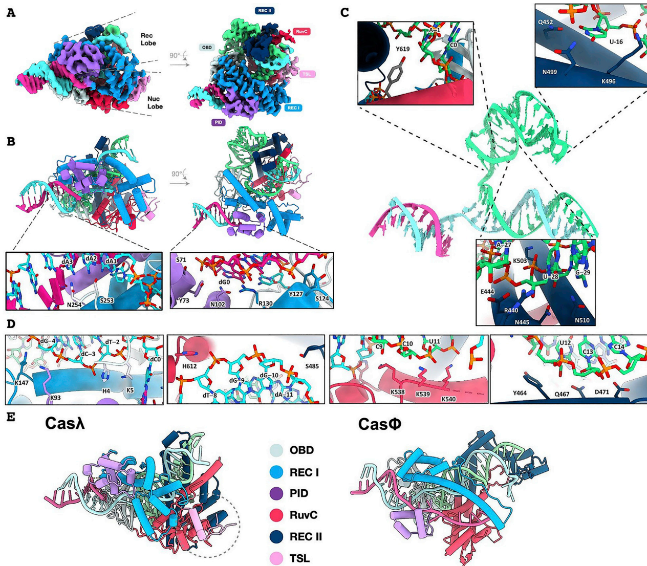
Figure S6. Structure of Casλ ternary complex, related to Figure 6
