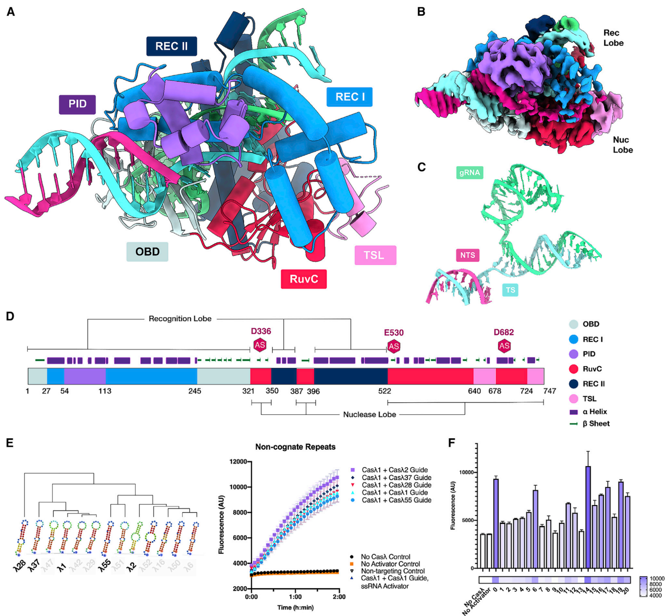
Figure 6. Structure of Casλ-gRNA-DNA complex
