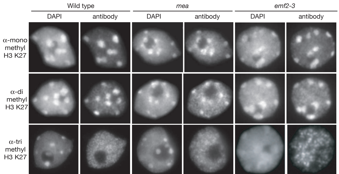
Figure S1. Distribution of mono-, di-, and tri-methyl H3K27 in two additional homozygous PcG mutants, mea and emf2-3 . Staining patterns in these mutants with the H3K27 methyl antibodies are unaffected as compared to the wild type.
