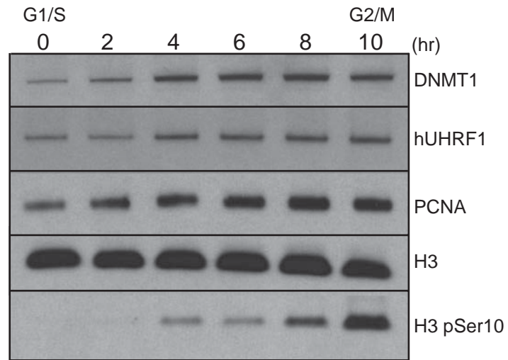
Figure S3. Cell cycle-dependent chromatin association of DNMT1, hUHRF1, and PCNA. HeLa cells were synchronized by thymidine/ aphidicolin block and released into regular medium. Time points in hours (hr) after the release are indicated at the top of the panels. Western blots for DNMT1, hUHRF, and PCNA to detect association with chromatin. H3 and H3 phospho-Ser10 (H3 pSer10) antibodies were used for a loading control and mitosis marker, respectively.
