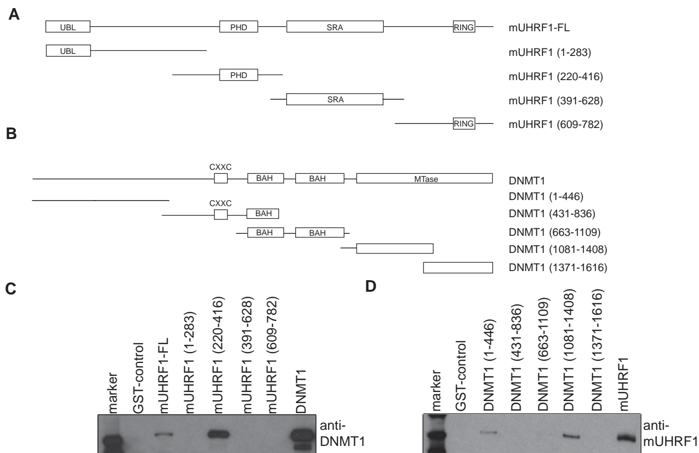
Figure S4. Mapping DNMT1 and mUHRF1 interaction domains. (A) Various domains of mUHRF1 are indicated by a schematic presentation of the GST fusion constructs shown with amino acid numbers. UBL, ubiquitin-like; PHD, plant homeodomain; SRA, SET and RING associated; RING, Really Interesting New Gene. (B) Various domains of DNMT1 are indicated by schematic diagram of the GST fusion fragments shown with amino acid numbers. CXXC, Zinc-finger; BAH, Bromo adjacent homology; MTase, methyltransferase. (C) GST pull-down assay demonstrating interacting regions between purified GST-fused UHRF1 fragments and baculovirus expressed full-length DNMT1. The input DNMT1 is included as control. All GST fusions were validated by western blot analysis with anti-GST antibodies (data not shown). After the transfer of the proteins, the blots were stained with ponceau stain (data not shown) to determine the quality of protein transfer. (D) GST pull-down assay demonstrating interacting regions between purified GST-fused DNMT1 fragments and E.coli expressed full-length 6xHis tagged UHRF1. The input mUHRF1 is included as control. All GST fusions were validated by western blot analysis with anti-GST antibodies (data not shown). After the transfer of the proteins, the blots were stained with ponceau stain (data not shown) to determine the quality of protein transfer.
