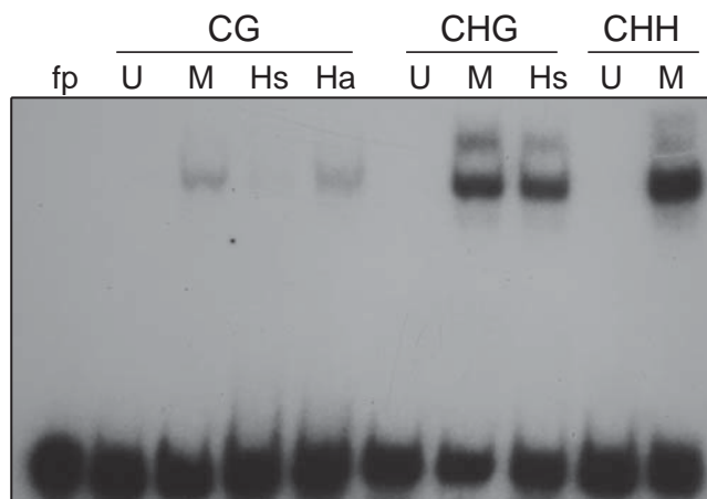
Figure S10. SuvH6 SRA binding specificity is different than mUHRF. Electrophoretic mobility shift assays with GST-SuvH6SRA binding to double-stranded oligonucleotides containing unmethylated (U), fully methylated (M), or hemi-methylated with the methyl-cytosine on the sense (Hs) or antisense (Ha) strand containing CG dinucleotides, CHG or CHH trinucleotides, where H = A, T, or C. fp is free probe.
