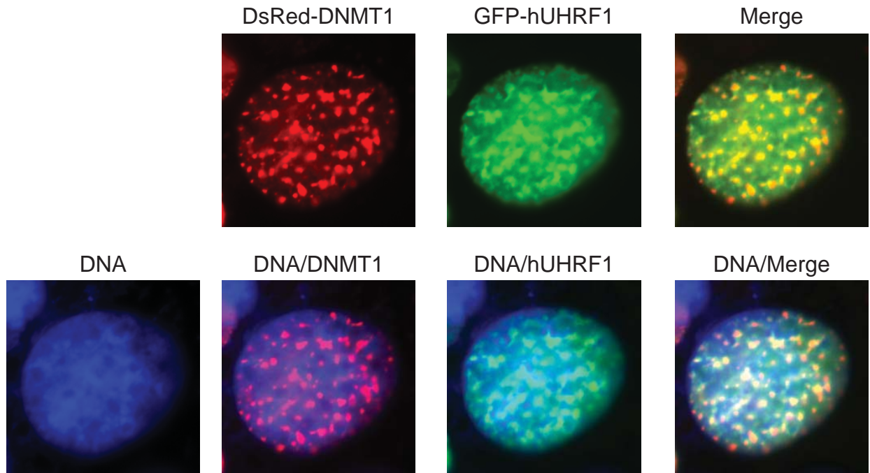
Figure S2. Colocalization of hUHRF1 and DNMT1. Detection of DsRed-DNMT1 and GFP-hUHRF1 transiently expressed in synchronized COS-7 cells. Cells were released from G1 arrest and visualized in late S Phase. DNA in the nucleus (DNA) was visualized with Hoechst stain.
