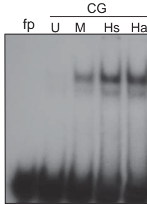
Figure S9. The SRA domain of hUHRF1 prefers hemimethylated DNA. Electrophoretic mobility shift assays with 100 ng of GST-hUHRF1 SRA domain binding to double-stranded oligonucleotides with CG dinucleotides either unmethylated (U), fully methylated (M), or hemimethylated on the sense (Hs) or antisense (Ha) strand. fp is free probe.
