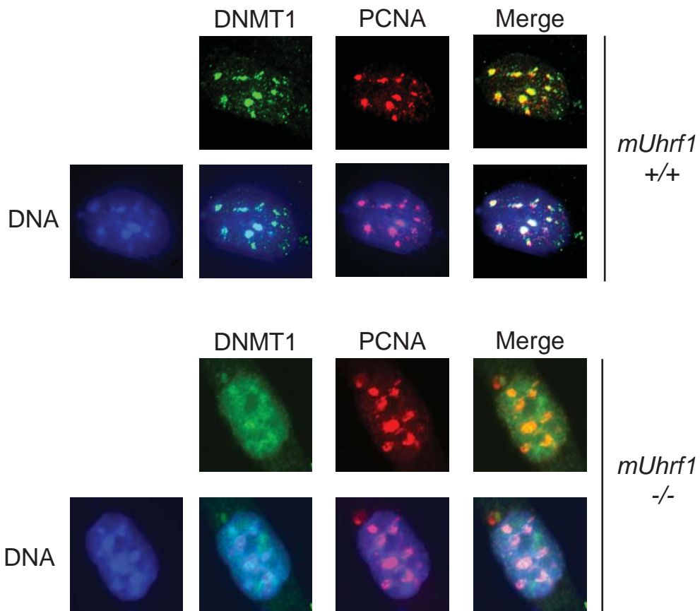
Figure S6. DNMT1 localization is disrupted in mUHRF1 -/- cells. Immunofluorescence images of wild-type (top panel) or mUhrf1 -/- (bottom panel) cells. DNMT1 localization was visualized with rabbit anti-DNMT1 antibodies and anti-rabbit AlexaFluor 488. PCNA was visualized with mouse anti-PCNA antibodies and anti-mouse AlexaFluor 594. The nuclear DNA was stained with Hoechst 33342 for visualization.
