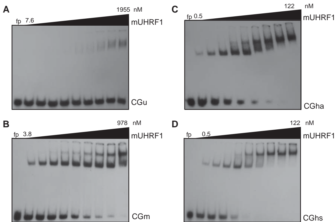
Figure S8. Binding Assays of mUHRF1 utilized for Figure 4B. Electrophoretic mobility shift assays with increasing amounts of GST-mUHRF1 binding unmethylated (CGu, A ), fully methylated (CGm, B ), or hemi-methylated (CGha, C ; CGhs, D ) double-stranded oligonucleotide, as representative of the data presented in Fig. 4B. Protein concentrations are doubled in each lane, starting at the left, with the lowest and highest amount indicated above the second and last lanes, respectively. fp is free probe.
