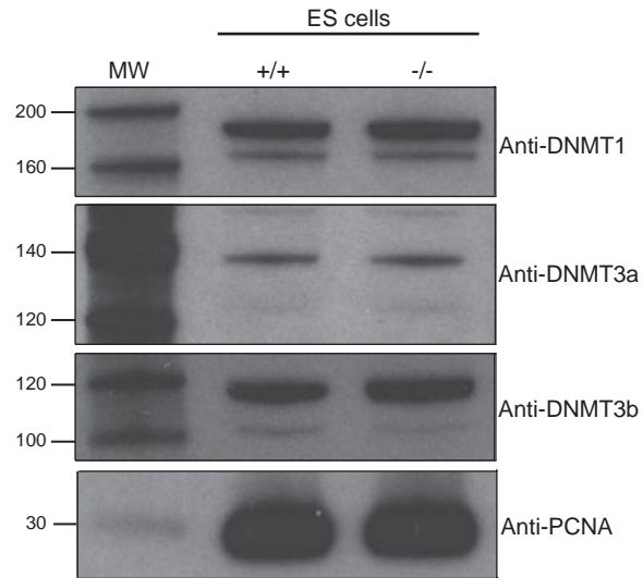
Figure S1. mUHRF1 -/- cells have wild-type levels of DNA methyltransferases. Western blot of DNMT1, DNMT3a, DNMT3b, and PCNA with cell extracts from wild-type (+/+) or mUHRF1 -/- (-/-) embryonic stem (ES) cells. MW denotes the lane with protein molecular weight markers, with sizes on left of gel in kDa.
