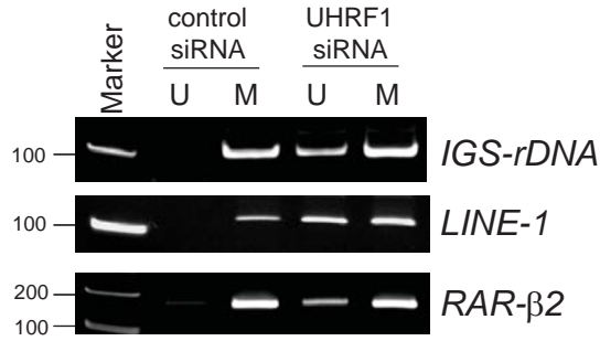
Figure S5. DNA Methylation levels are decreased by UHRF1 knockdown in HeLa cells. Methylation-specific PCR for IGS-rDNA , LINE-1 , and RAR-β2 after siRNA-mediated knockdown of hUHRF1 in HeLa cells. Unmethylated (U) and methylated (M) gene-specific products are shown. Markers are in basepairs.
